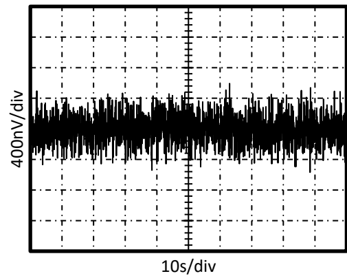
0.01Hz TO 10Hz NOISE AT V_S = 2.9\text{V}
